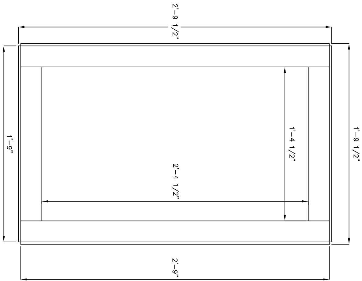
BASE TRAY TOP VIEW
